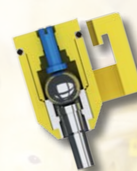
Revolution Nipple
