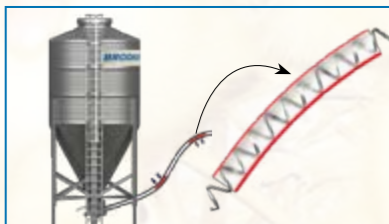
Single unloader shown with optional swing away bottom for 100% clean out.
